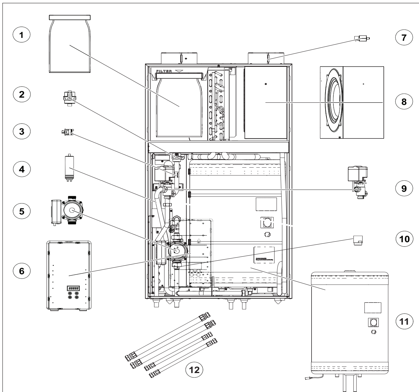
Fig.3 Exploded view met servicebare delen Combi 50
