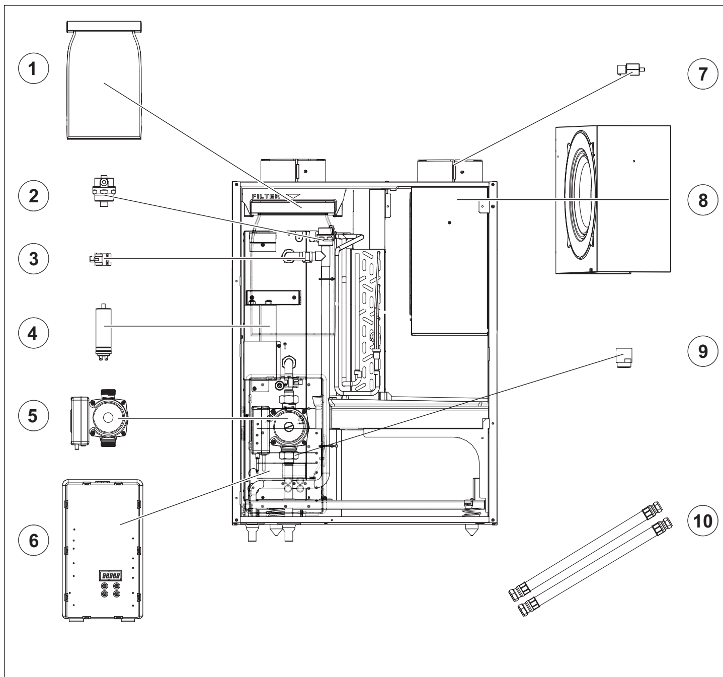
Fig.4 Exploded view met servicebare delen Solo
